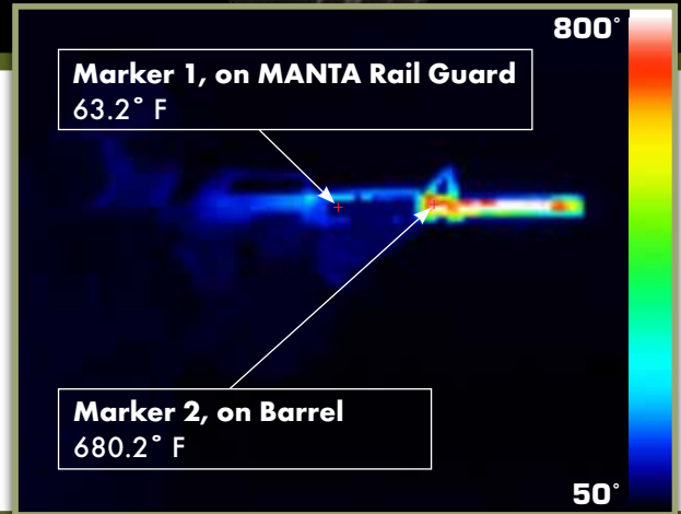
Thermal image after 210 consecutive rounds.
